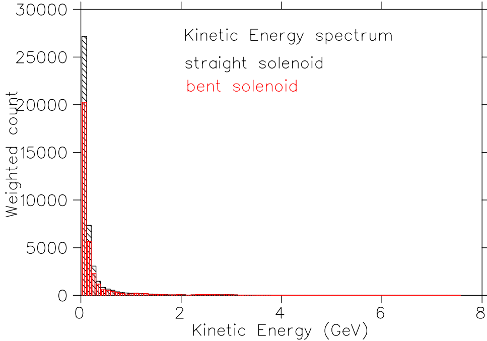
FIG. 7. [color] Energy spectrum of protons with and without bent solenoid at the end of the bent solenoid; each bin corresponds to 100 MeV.
